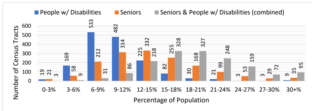
Figure 2: Count of Census Tracts by Percentage of Population
